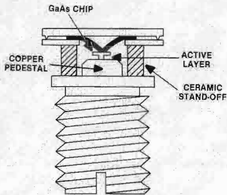
Packaged Gunn diode as presented in literature from Microwave Associates.
