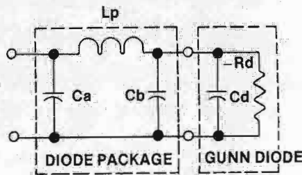
Equivalent circuit of a Gunn diode. The parasitic reactances of the diode package are included.
