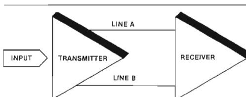
Figure 2. Block representation of A and B in RS-422 interface. Note that A < B = \text{mark} or "1," and A > B = \text{space} or "0."
