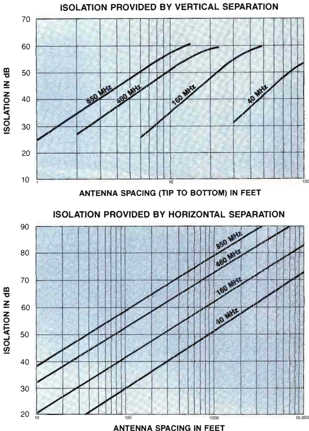
Figure 5. Separating the receive antenna from other transmitting antennas will often provide the needed isolation. The tower and other structures can have a significant impact on the actual isolation encountered.
